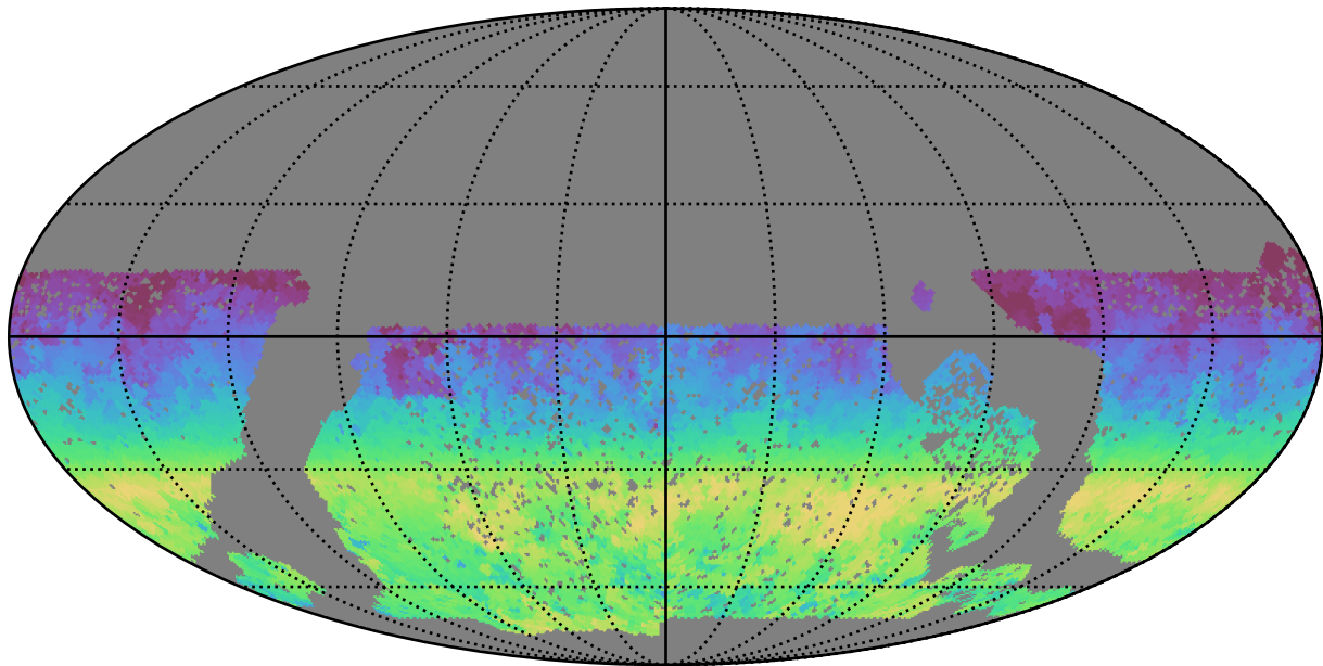
baseline_v3.0_10yrs WFD i band: AngleRange rotSkyPos
