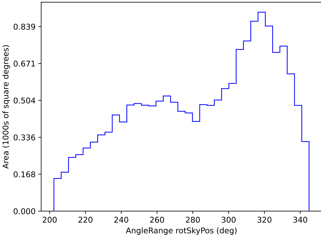
baseline_v3.0_10yrs WFD i band: AngleRange rotSkyPos
