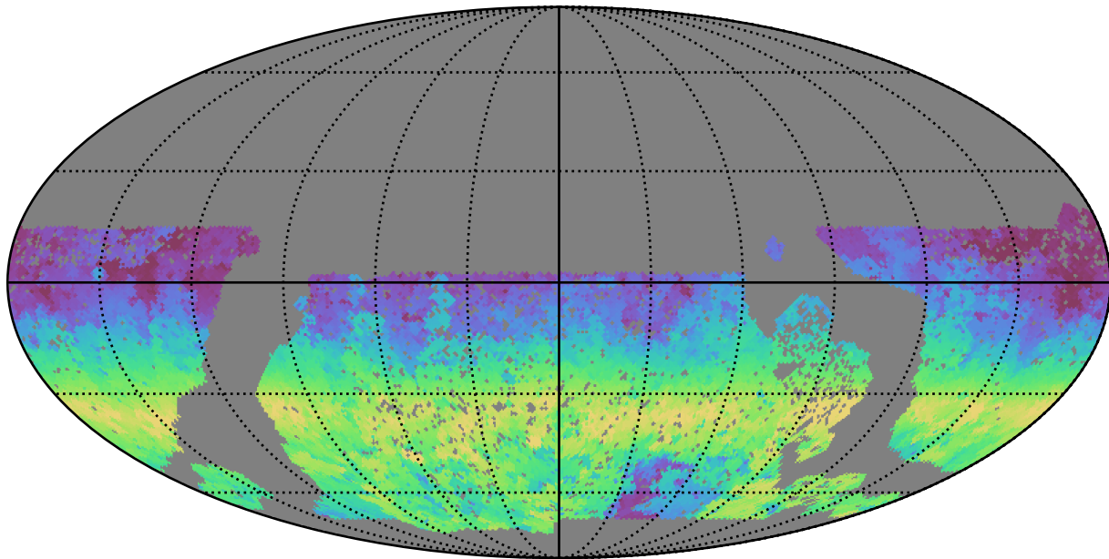
baseline_v3.0_10yrs WFD g band: AngleRange rotSkyPos
