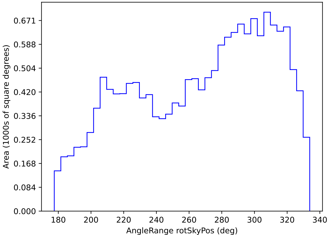
baseline_v3.0_10yrs WFD g band: AngleRange rotSkyPos
