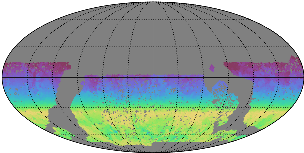
baseline_v3.0_10yrs WFD all bands: AngleRange rotSkyPos
