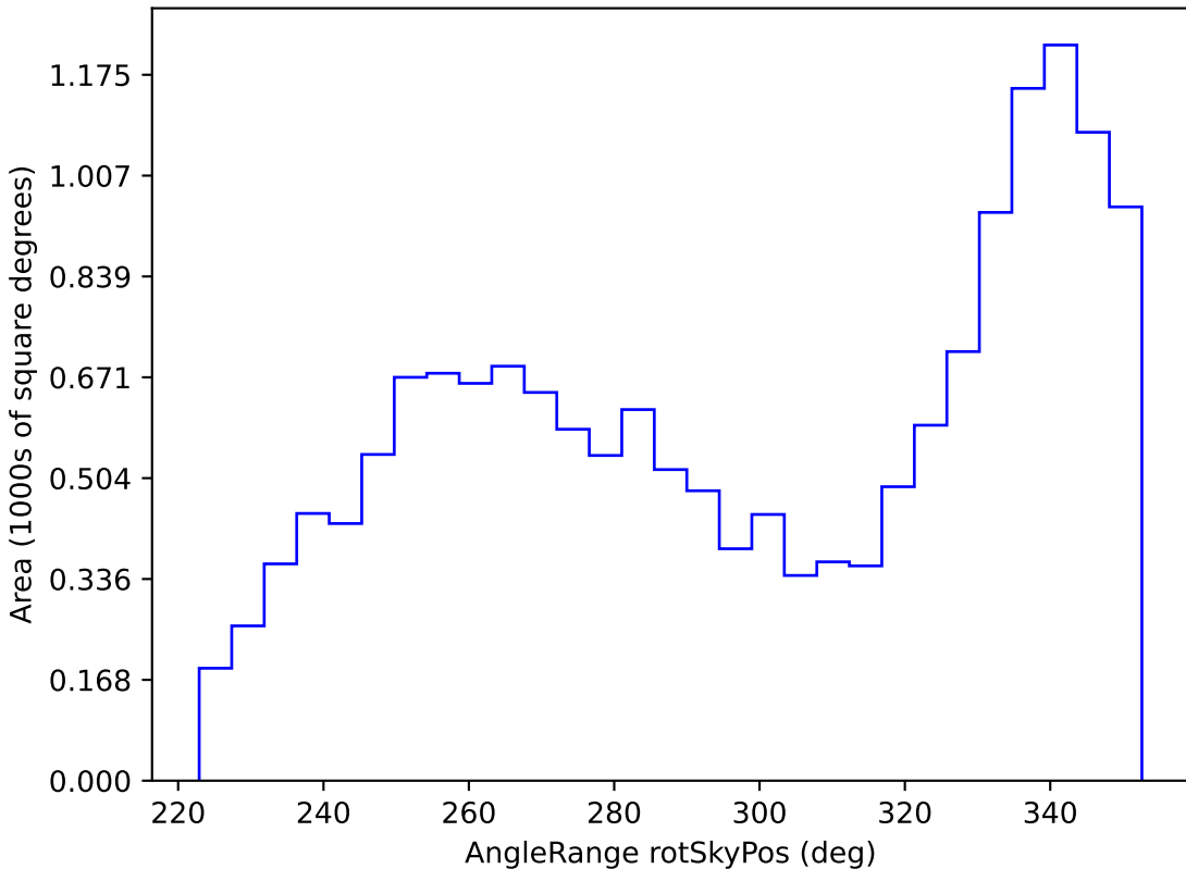
baseline_v3.0_10yrs WFD all bands: AngleRange rotSkyPos
