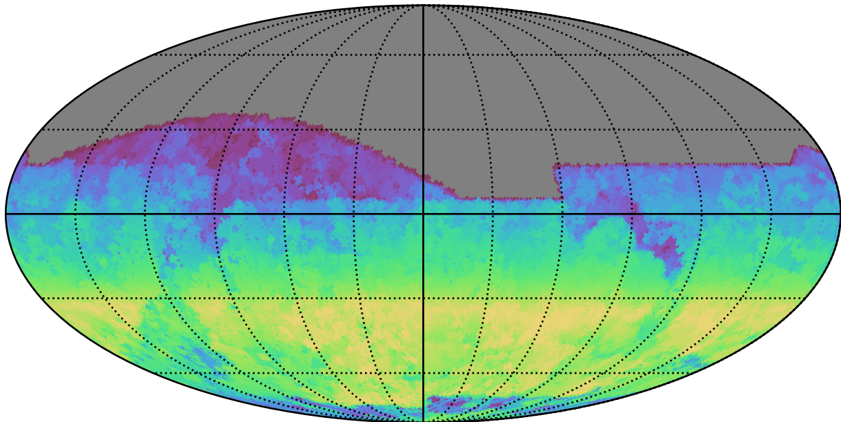
baseline_v3.0_10yrs All sky z band: AngleRange rotSkyPos
