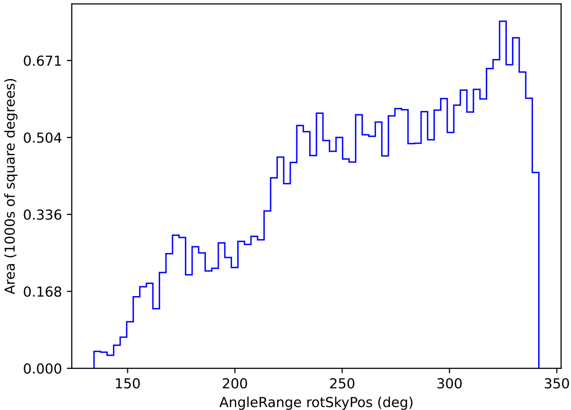
baseline_v3.0_10yrs All sky z band: AngleRange rotSkyPos
