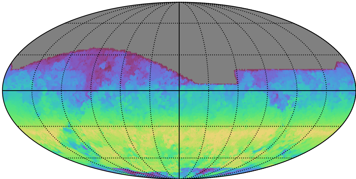
baseline_v3.0_10yrs All sky r band: AngleRange rotSkyPos
