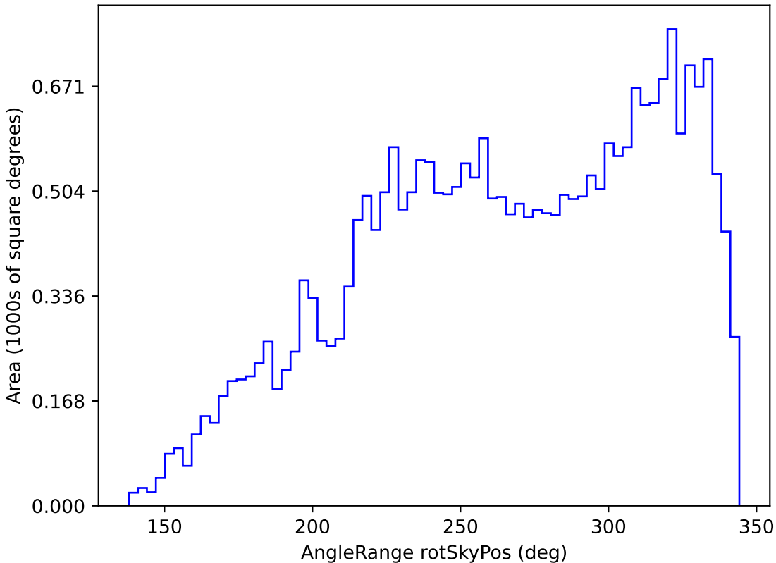
baseline_v3.0_10yrs All sky r band: AngleRange rotSkyPos
