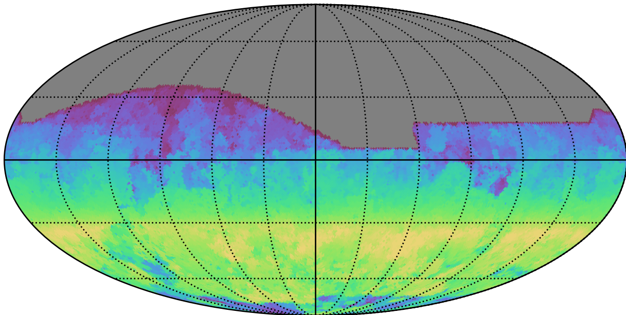
baseline_v3.0_10yrs All sky i band: AngleRange rotSkyPos
