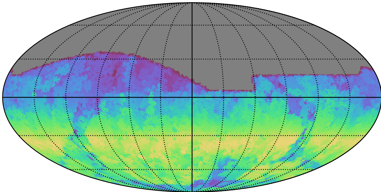
baseline_v3.0_10yrs All sky g band: AngleRange rotSkyPos
