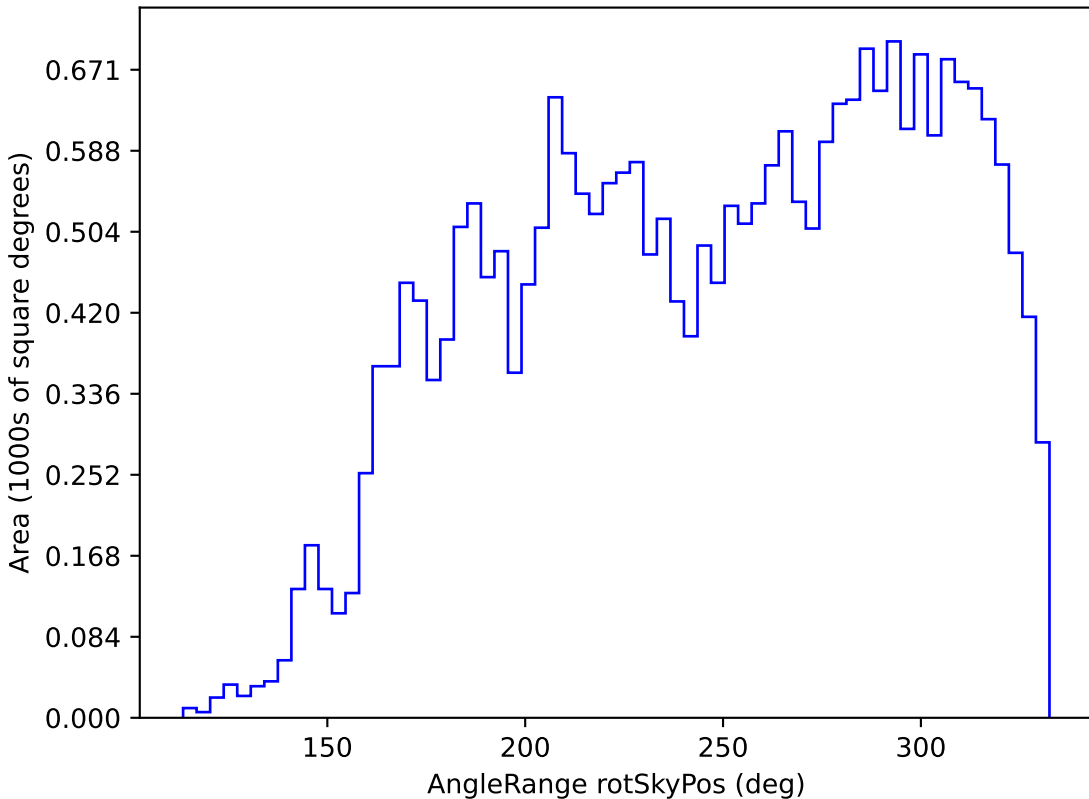
baseline_v3.0_10yrs All sky g band: AngleRange rotSkyPos
