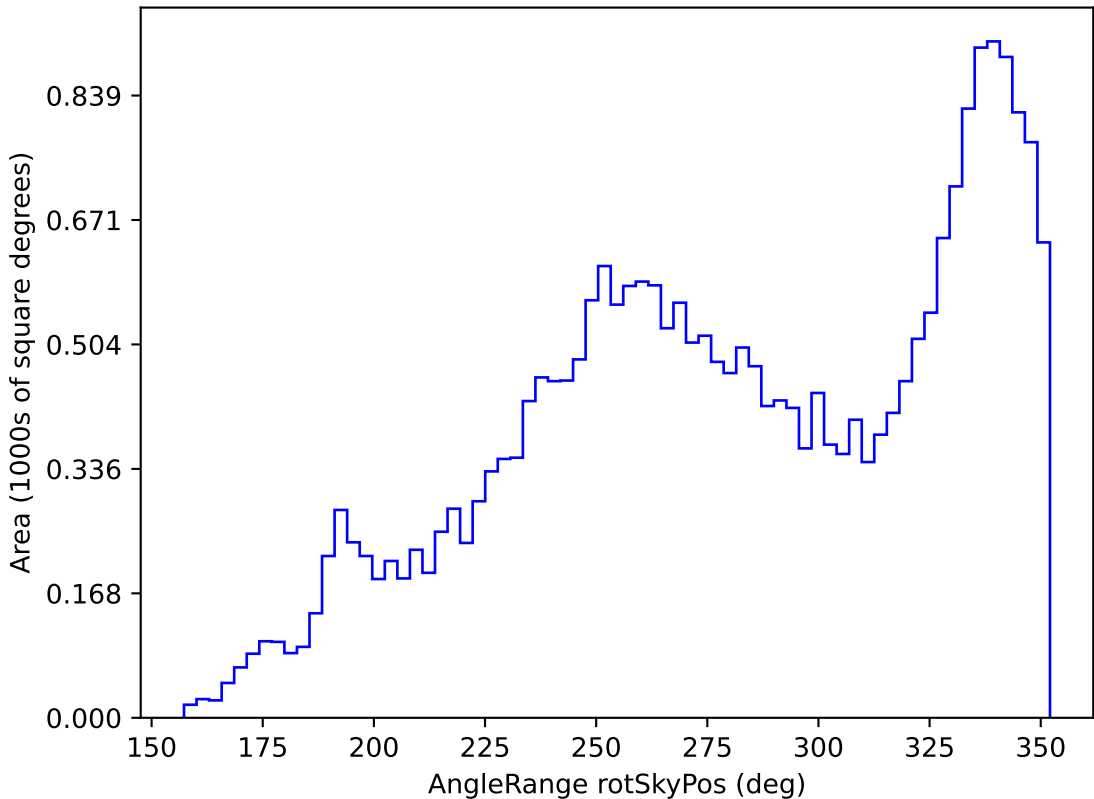
baseline_v3.0_10yrs All sky all bands: AngleRange rotSkyPos
