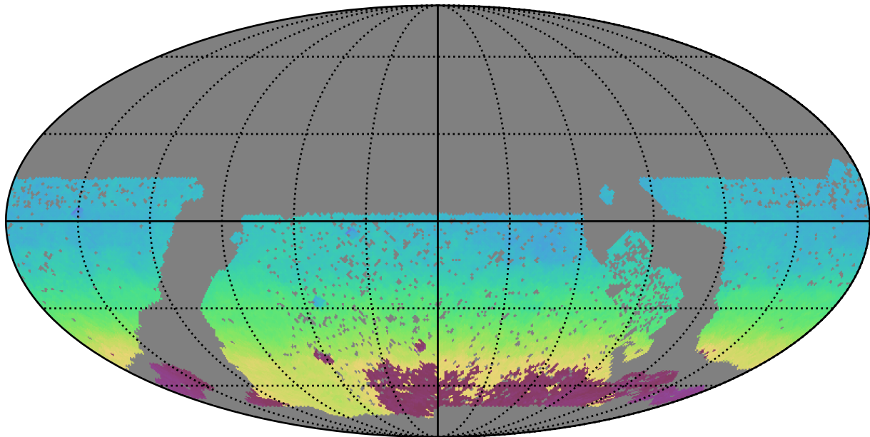
baseline_v3.0_10yrs WFD z band: AngleMean rotSkyPos
