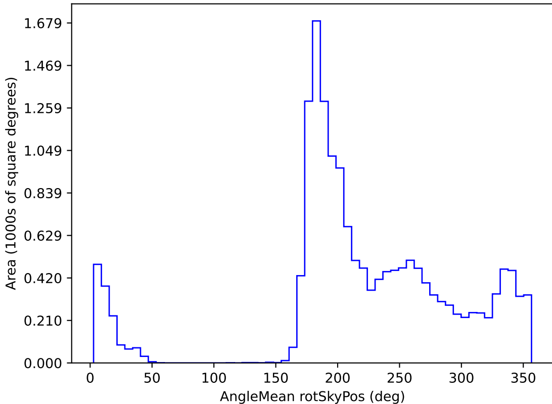
baseline_v3.0_10yrs WFD z band: AngleMean rotSkyPos
