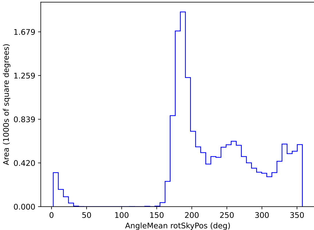
baseline_v3.0_10yrs WFD y band: AngleMean rotSkyPos
