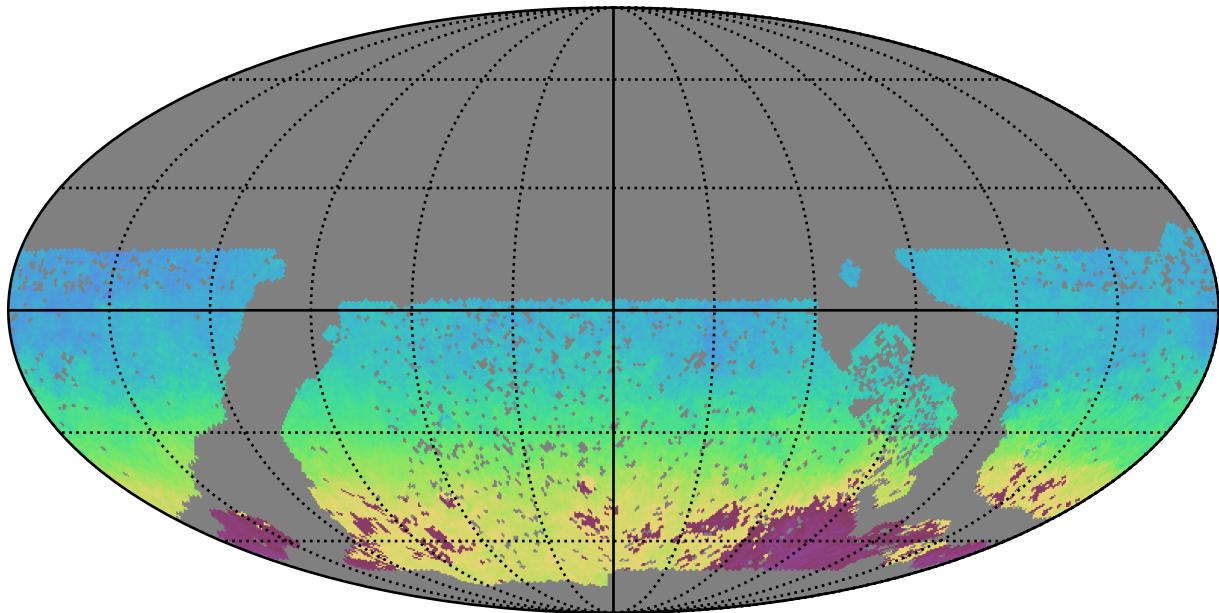
baseline_v3.0_10yrs WFD u band: AngleMean rotSkyPos
