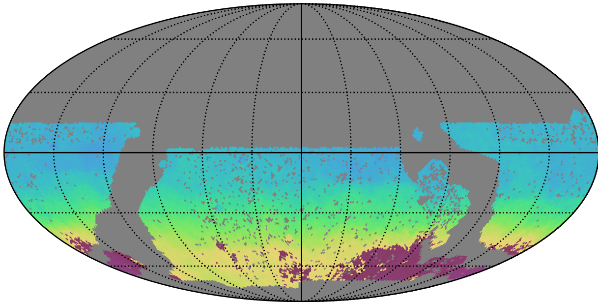
baseline_v3.0_10yrs WFD r band: AngleMean rotSkyPos
