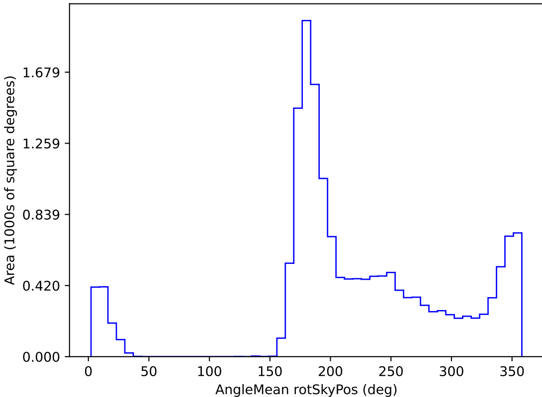
baseline_v3.0_10yrs WFD r band: AngleMean rotSkyPos
