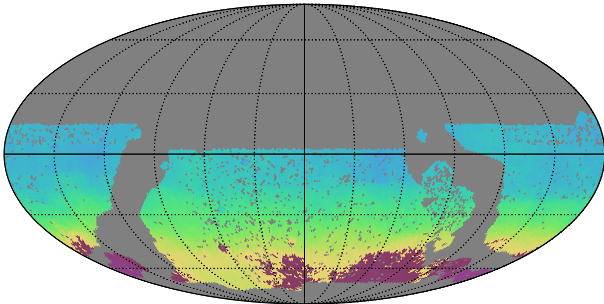
baseline_v3.0_10yrs WFD i band: AngleMean rotSkyPos
