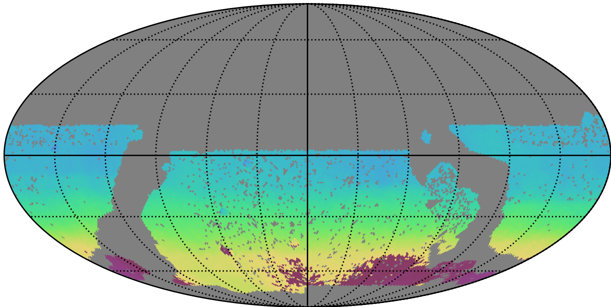
baseline_v3.0_10yrs WFD all bands: AngleMean rotSkyPos
