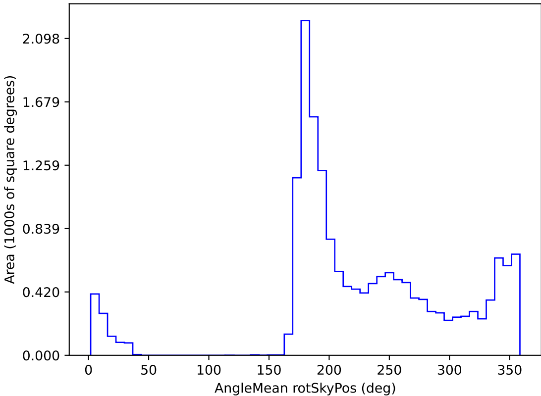
baseline_v3.0_10yrs WFD all bands: AngleMean rotSkyPos
