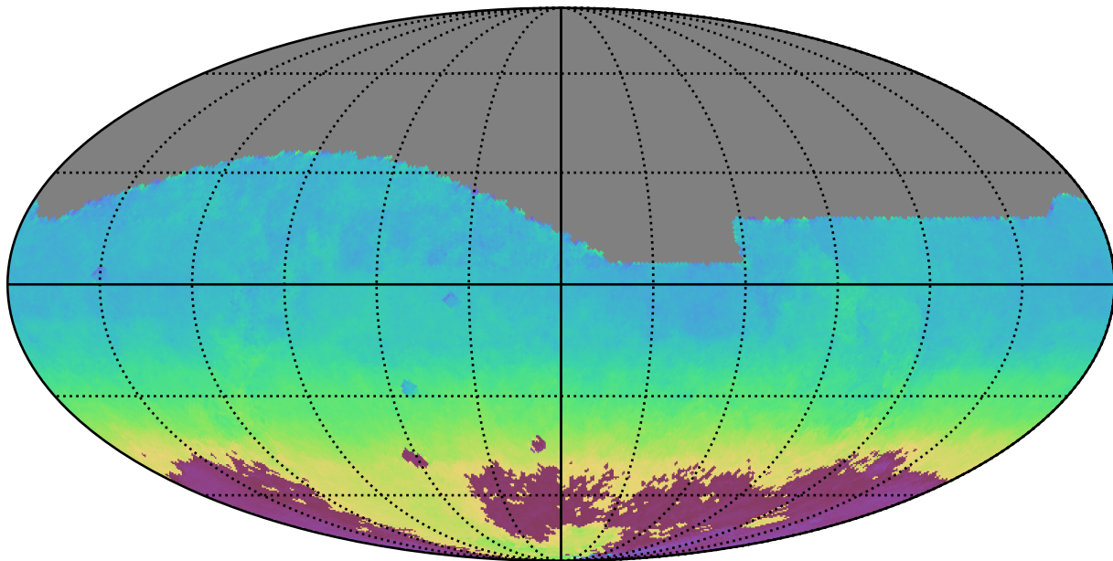
baseline_v3.0_10yrs All sky z band: AngleMean rotSkyPos
