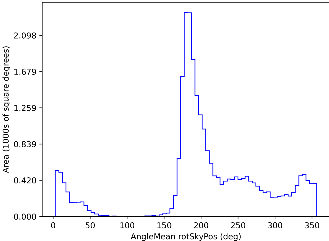
baseline_v3.0_10yrs All sky z band: AngleMean rotSkyPos
