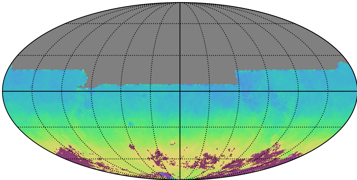
baseline_v3.0_10yrs All sky y band: AngleMean rotSkyPos
