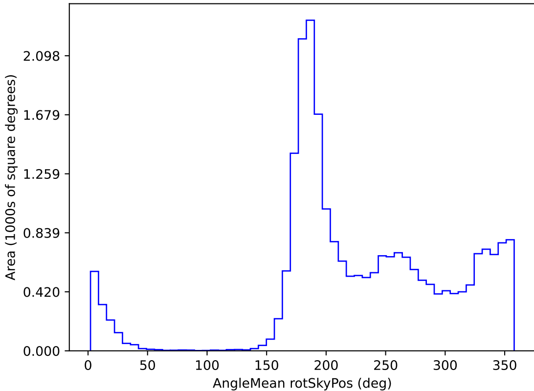
baseline_v3.0_10yrs All sky y band: AngleMean rotSkyPos
