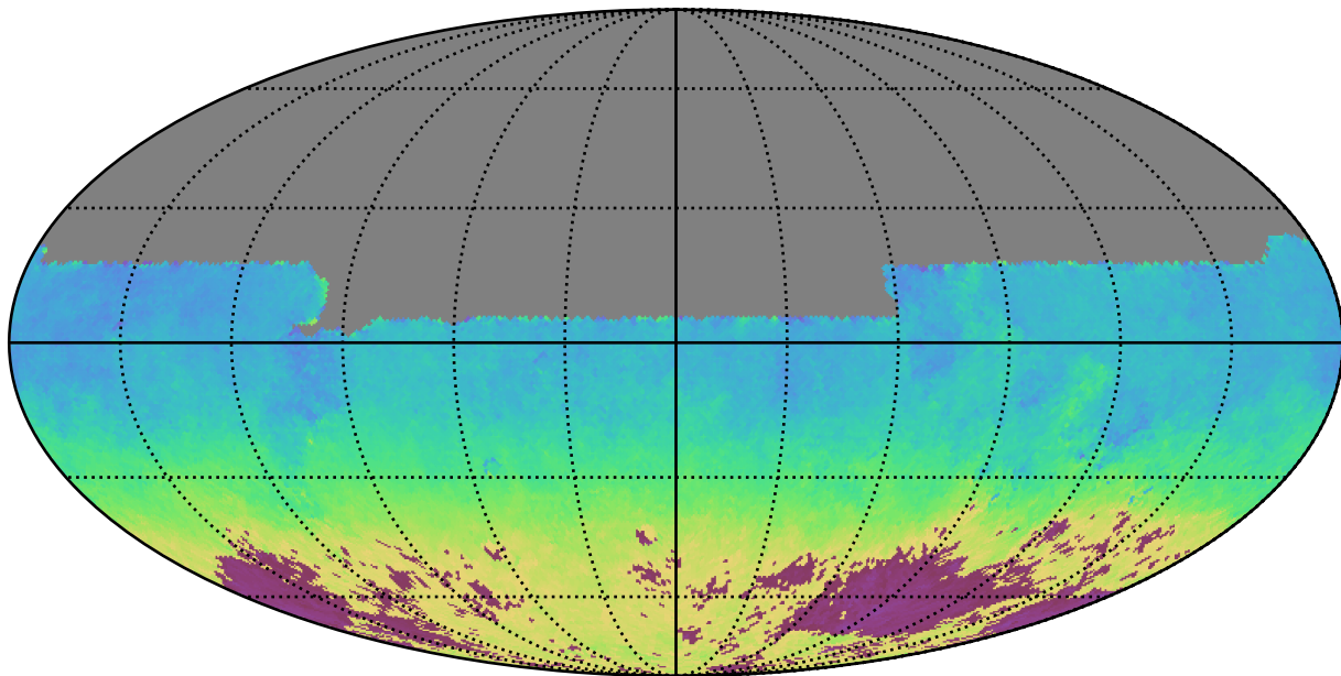
baseline_v3.0_10yrs All sky u band: AngleMean rotSkyPos
