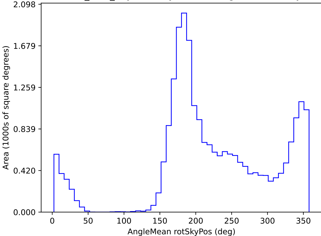
baseline_v3.0_10yrs All sky u band: AngleMean rotSkyPos
