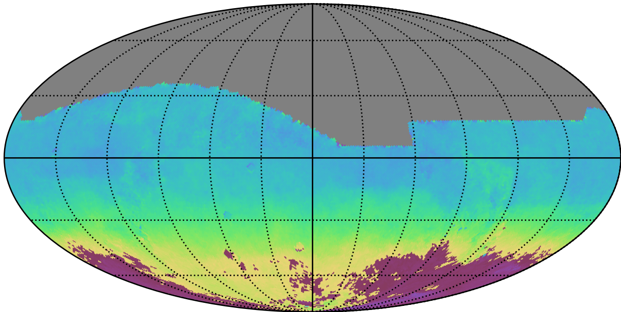
baseline_v3.0_10yrs All sky r band: AngleMean rotSkyPos
