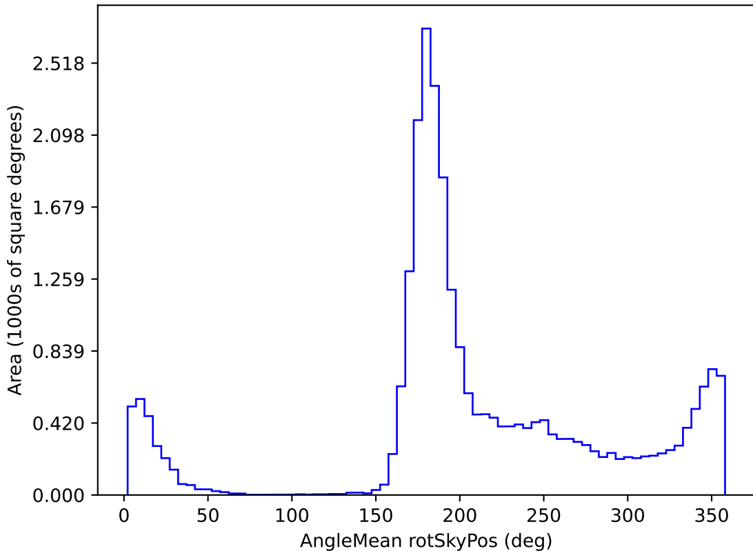
baseline_v3.0_10yrs All sky r band: AngleMean rotSkyPos
