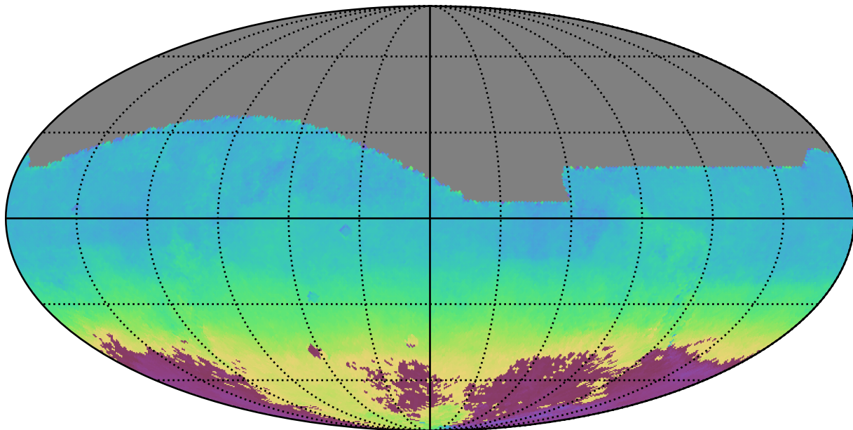
baseline_v3.0_10yrs All sky i band: AngleMean rotSkyPos
