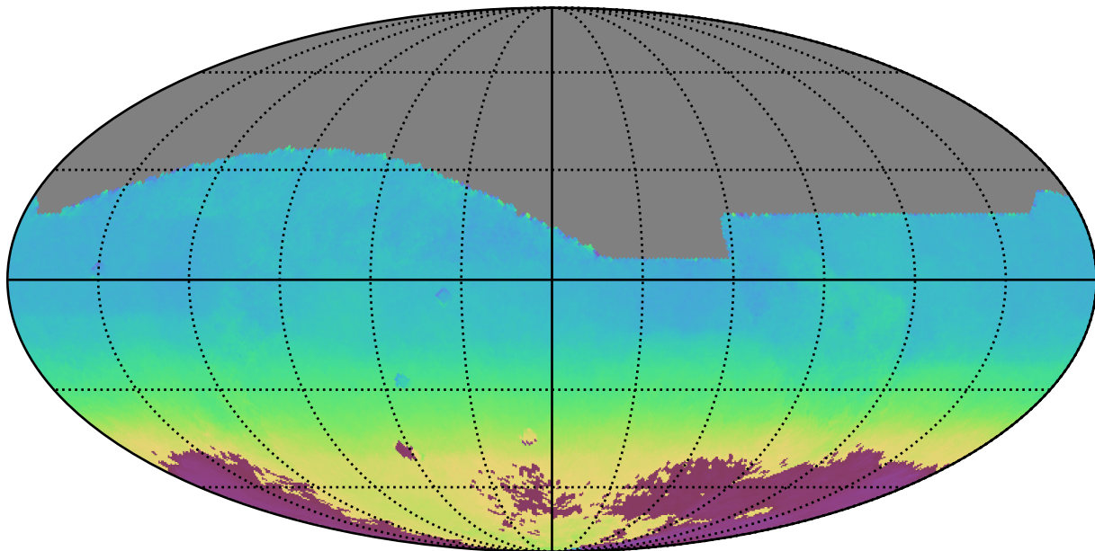
baseline_v3.0_10yrs All sky all bands: AngleMean rotSkyPos
