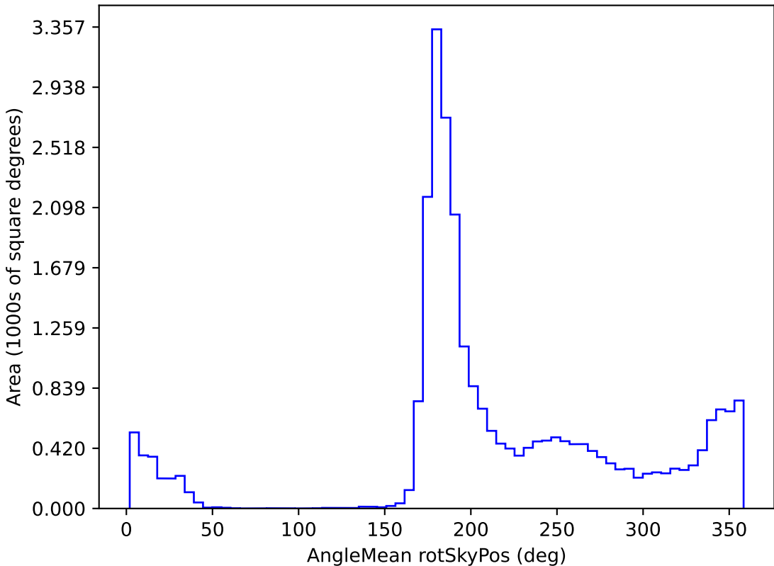
baseline_v3.0_10yrs All sky all bands: AngleMean rotSkyPos
