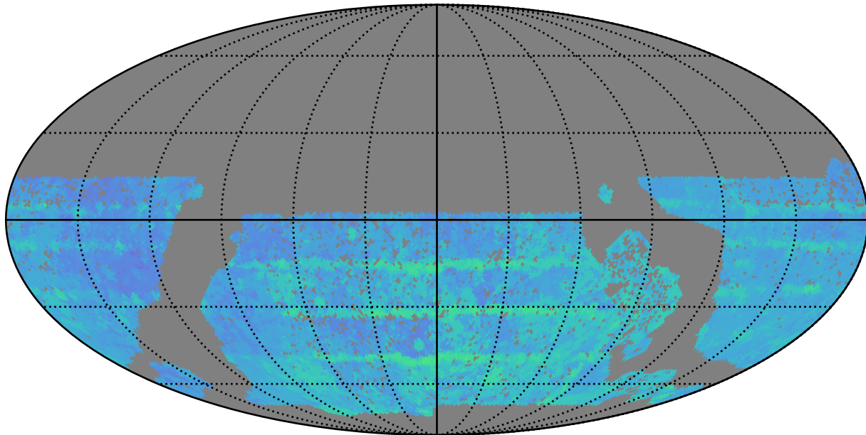
baseline_v3.0_10yrs WFD z band: 80thPercentile Season Length
