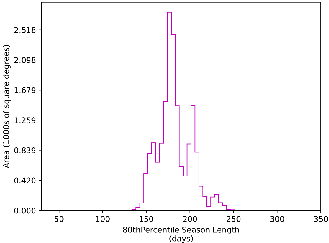
baseline_v3.0_10yrs WFD z band: 80thPercentile Season Length
