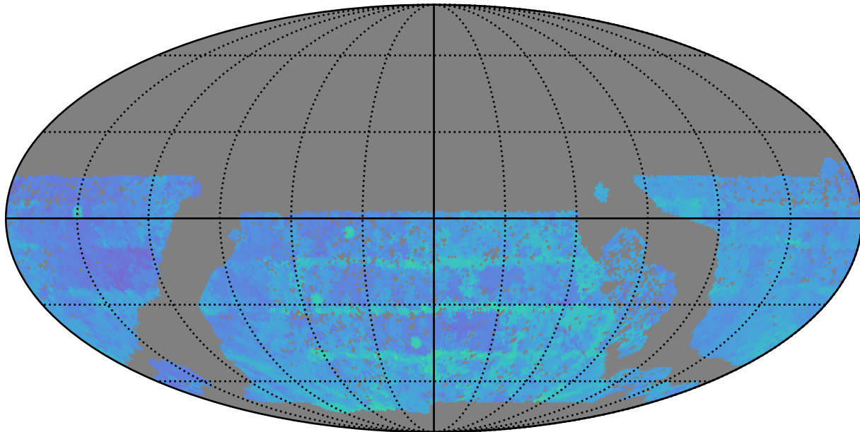
baseline_v3.0_10yrs WFD y band: 80thPercentile Season Length
