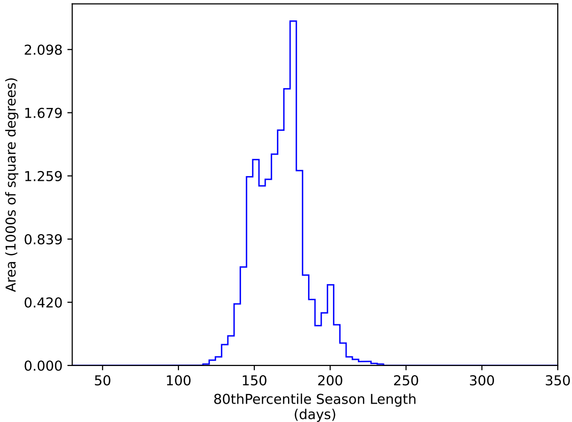
baseline_v3.0_10yrs WFD y band: 80thPercentile Season Length
