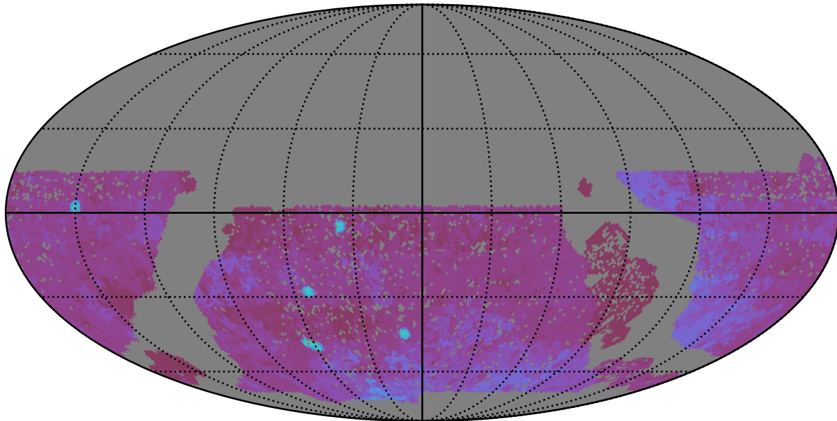
baseline_v3.0_10yrs WFD u band: 80thPercentile Season Length
