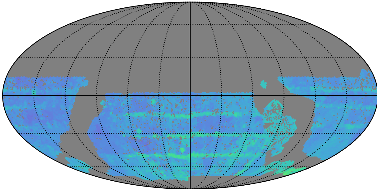
baseline_v3.0_10yrs WFD r band: 80thPercentile Season Length
