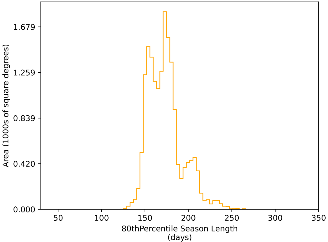
baseline_v3.0_10yrs WFD r band: 80thPercentile Season Length
