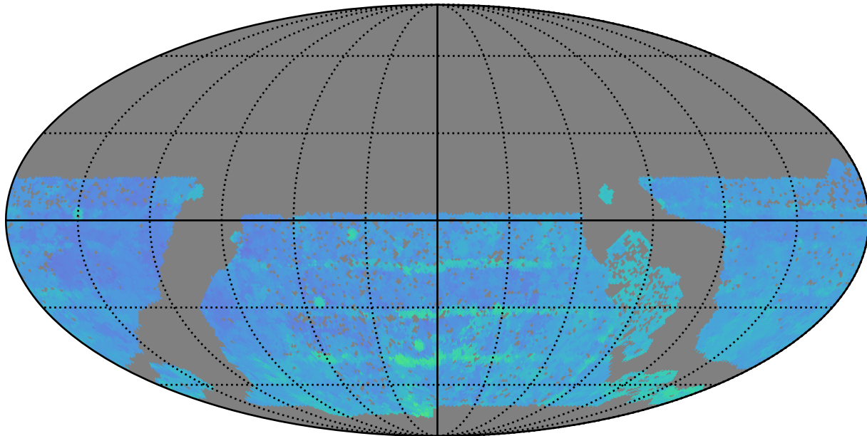
baseline_v3.0_10yrs WFD i band: 80thPercentile Season Length
