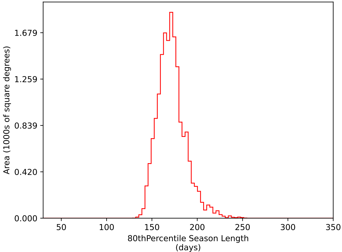
baseline_v3.0_10yrs WFD i band: 80thPercentile Season Length
