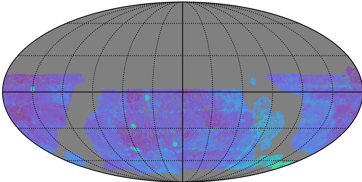
baseline_v3.0_10yrs WFD g band: 80thPercentile Season Length
