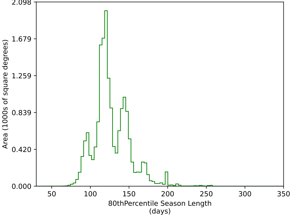
baseline_v3.0_10yrs WFD g band: 80thPercentile Season Length
