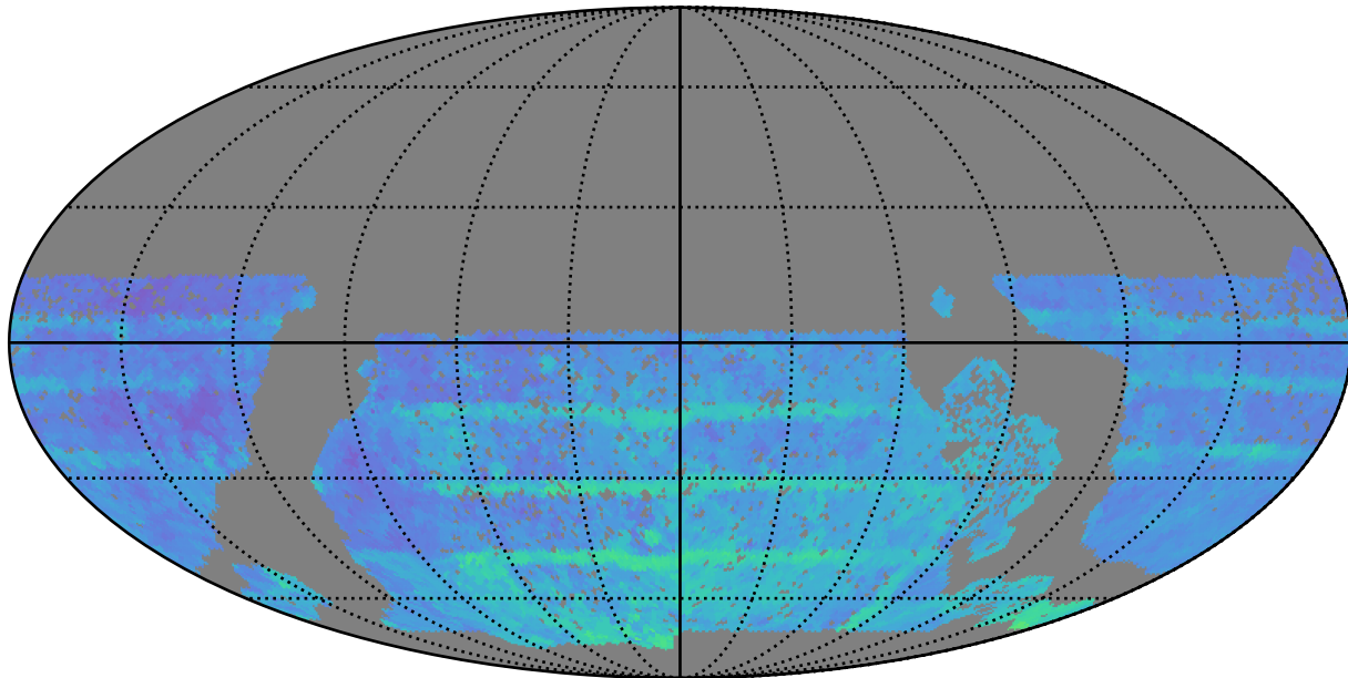
baseline_v3.0_10yrs WFD all bands: 80thPercentile Season Length
