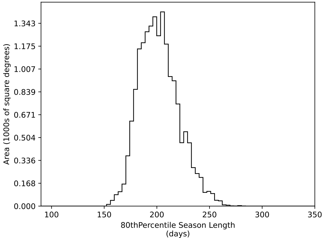
baseline_v3.0_10yrs WFD all bands: 80thPercentile Season Length
