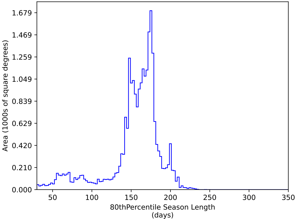
baseline_v3.0_10yrs All sky y band: 80thPercentile Season Length
