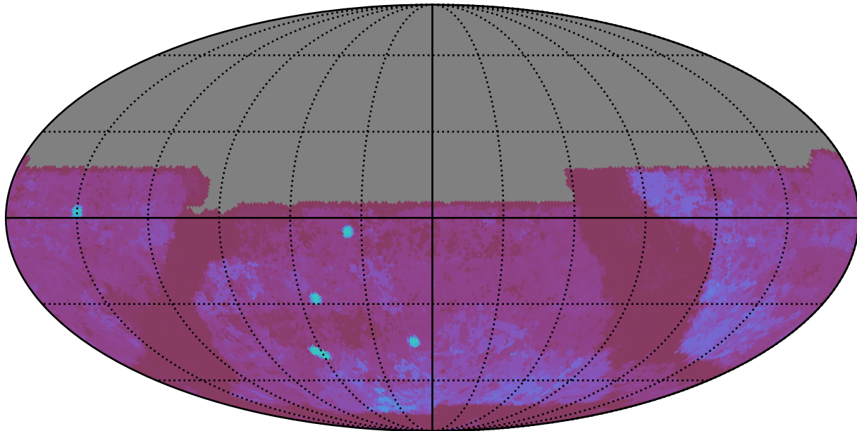
baseline_v3.0_10yrs All sky u band: 80thPercentile Season Length
