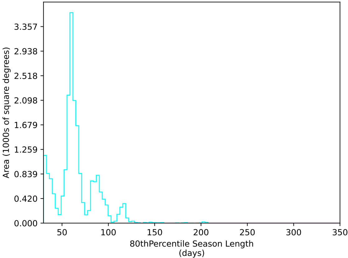
baseline_v3.0_10yrs All sky u band: 80thPercentile Season Length
